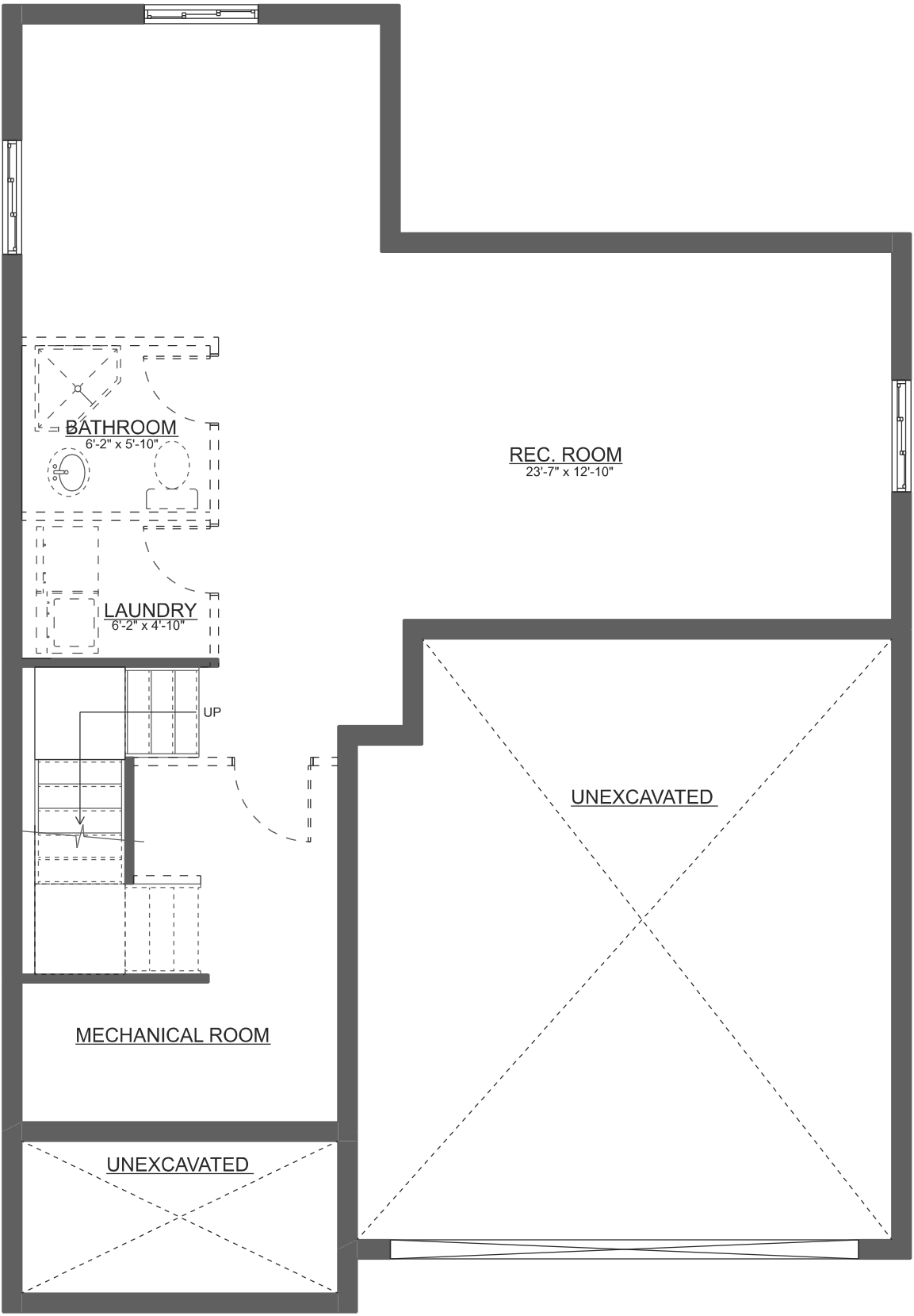
BASEMENT PLAN
