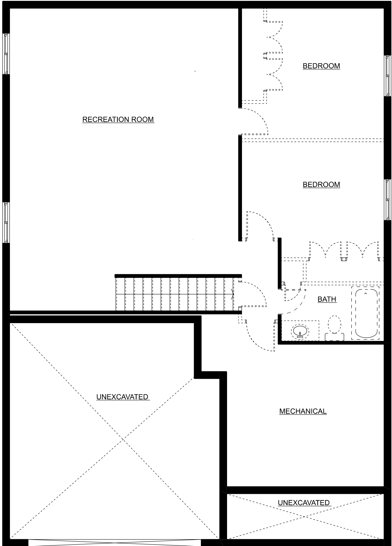
BASEMENT PLAN
