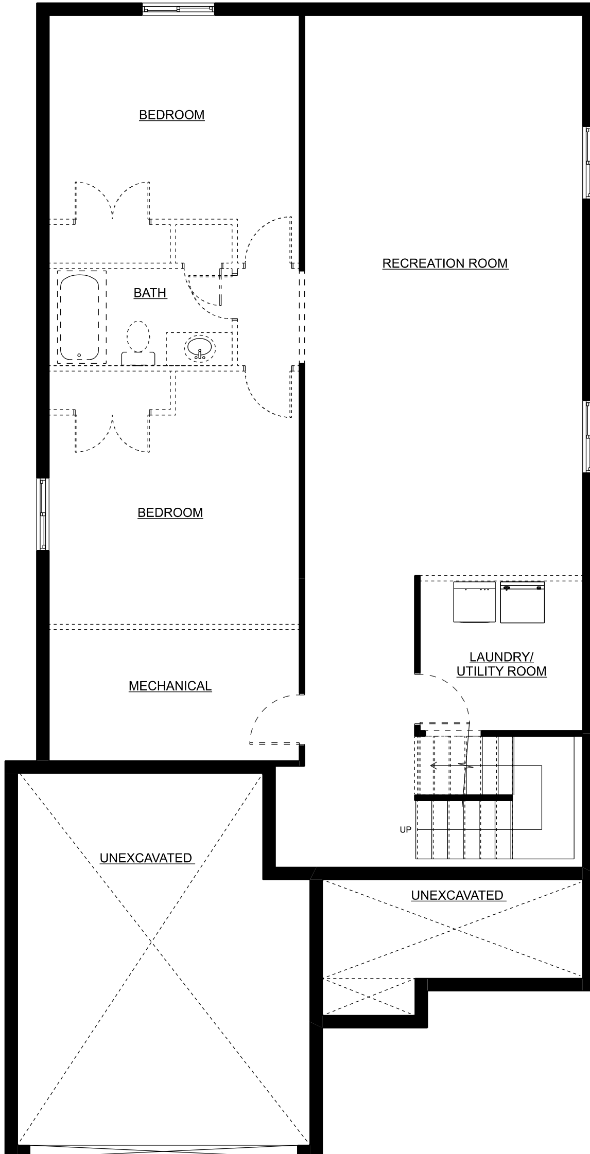
BASEMENT PLAN
