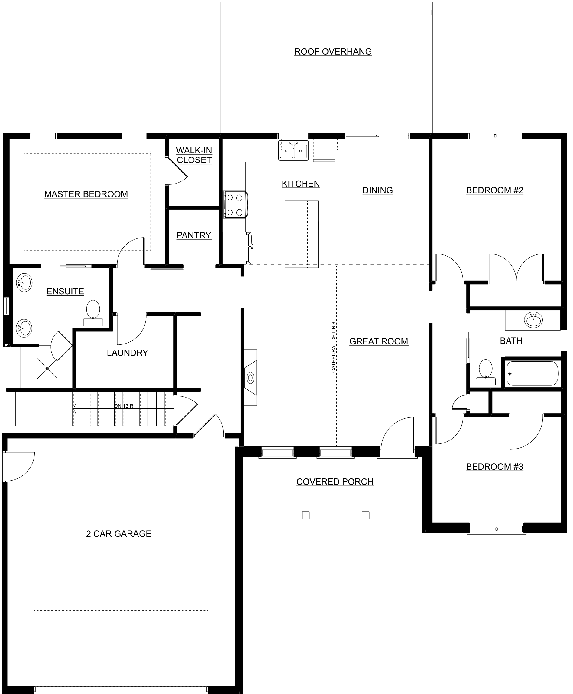
MAIN FLOOR PLAN SCALE: 3/16" = 1'-0"
