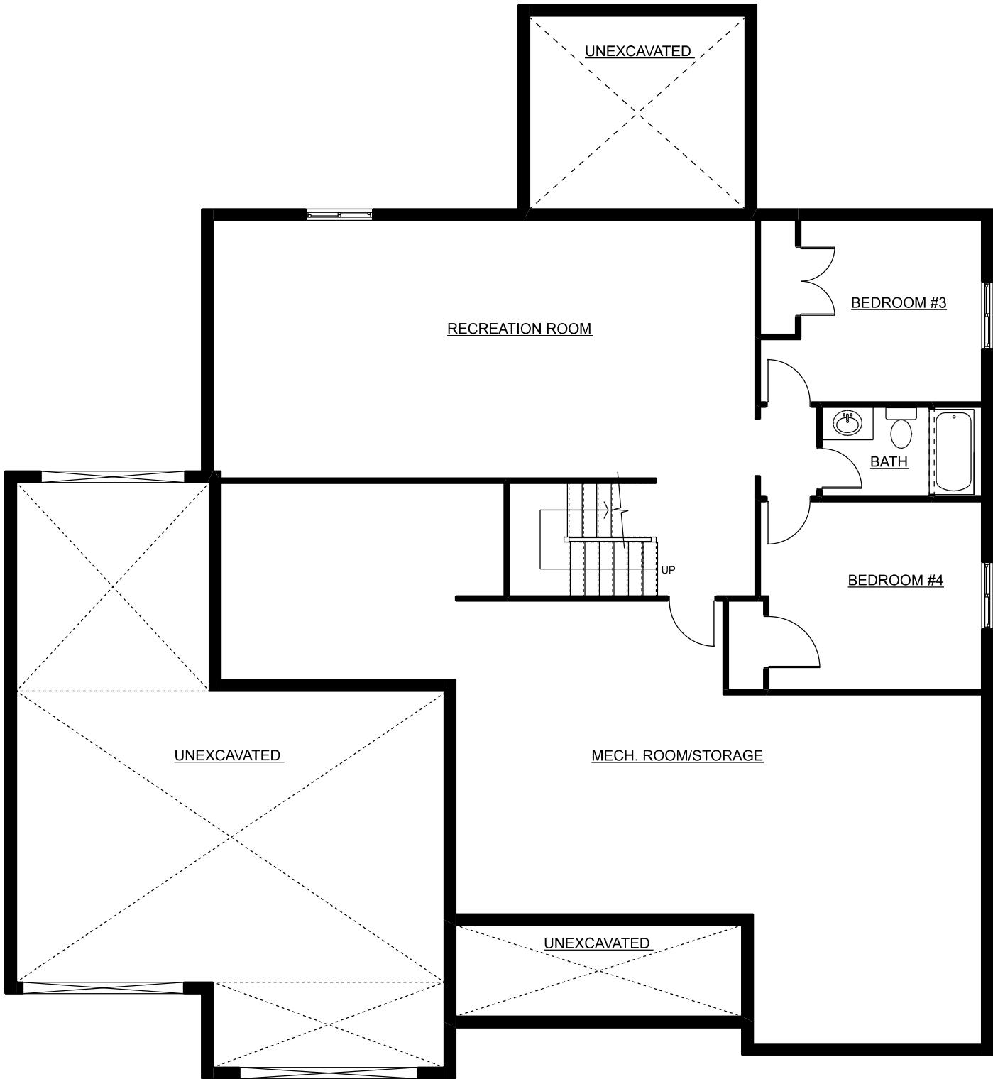
BASEMENT PLAN
