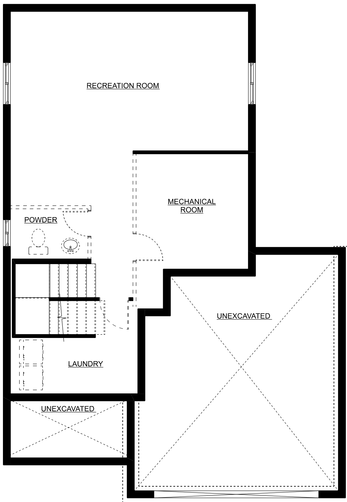
BASEMENT PLAN
