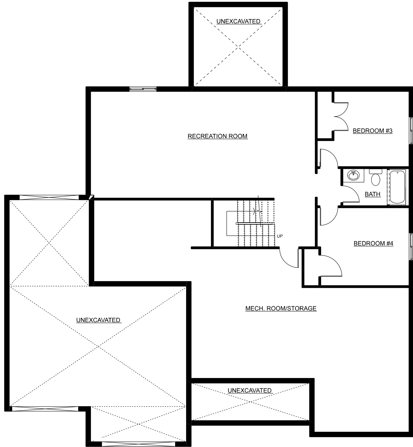
BASEMENT PLAN
