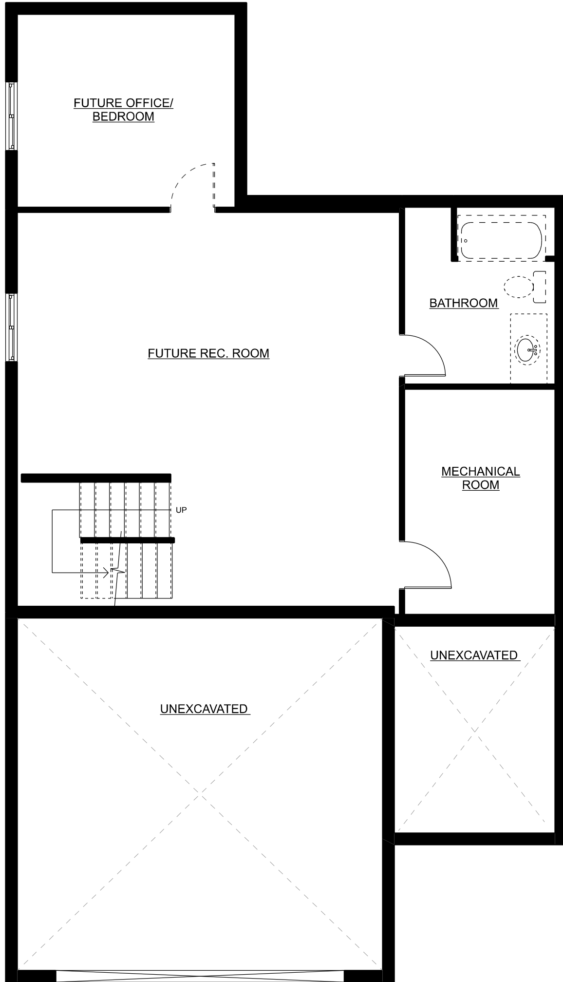
BASEMENT PLAN
