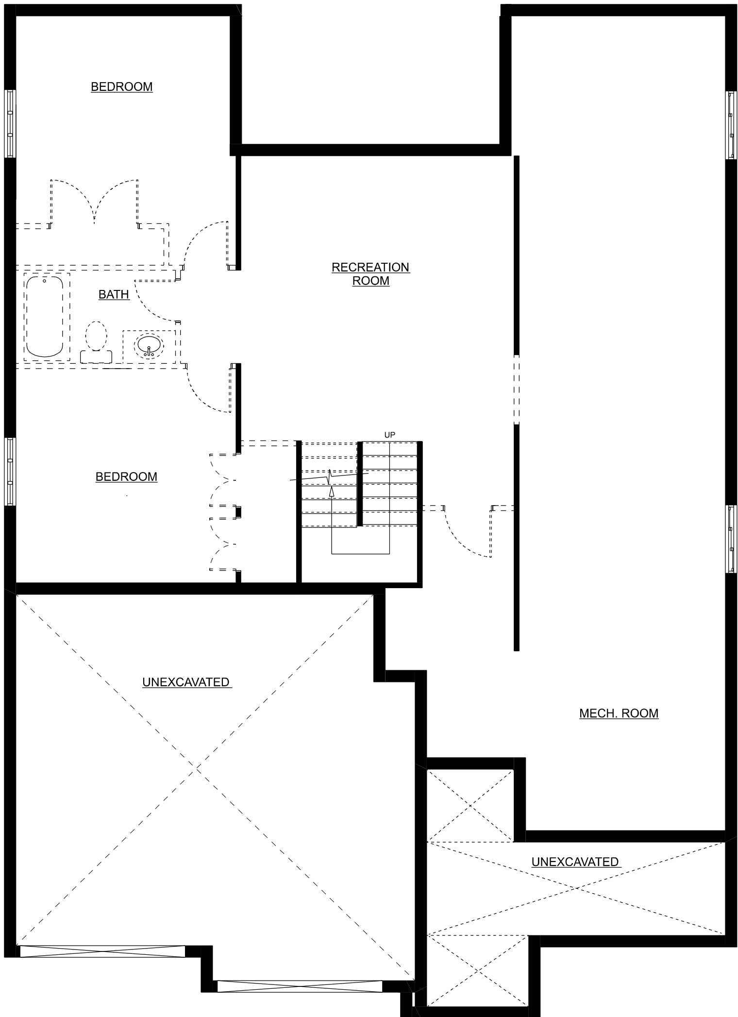
BASEMENT PLAN
