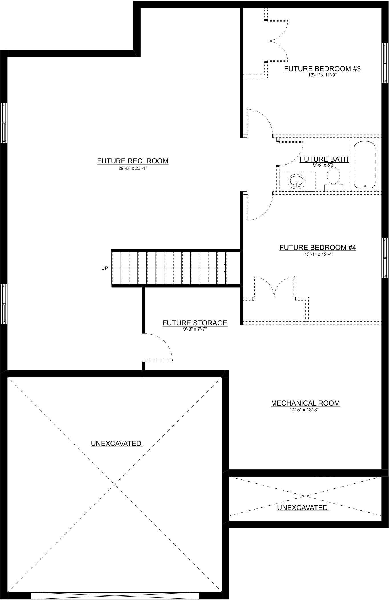
BASEMENT PLAN (NOT FINISHED)
