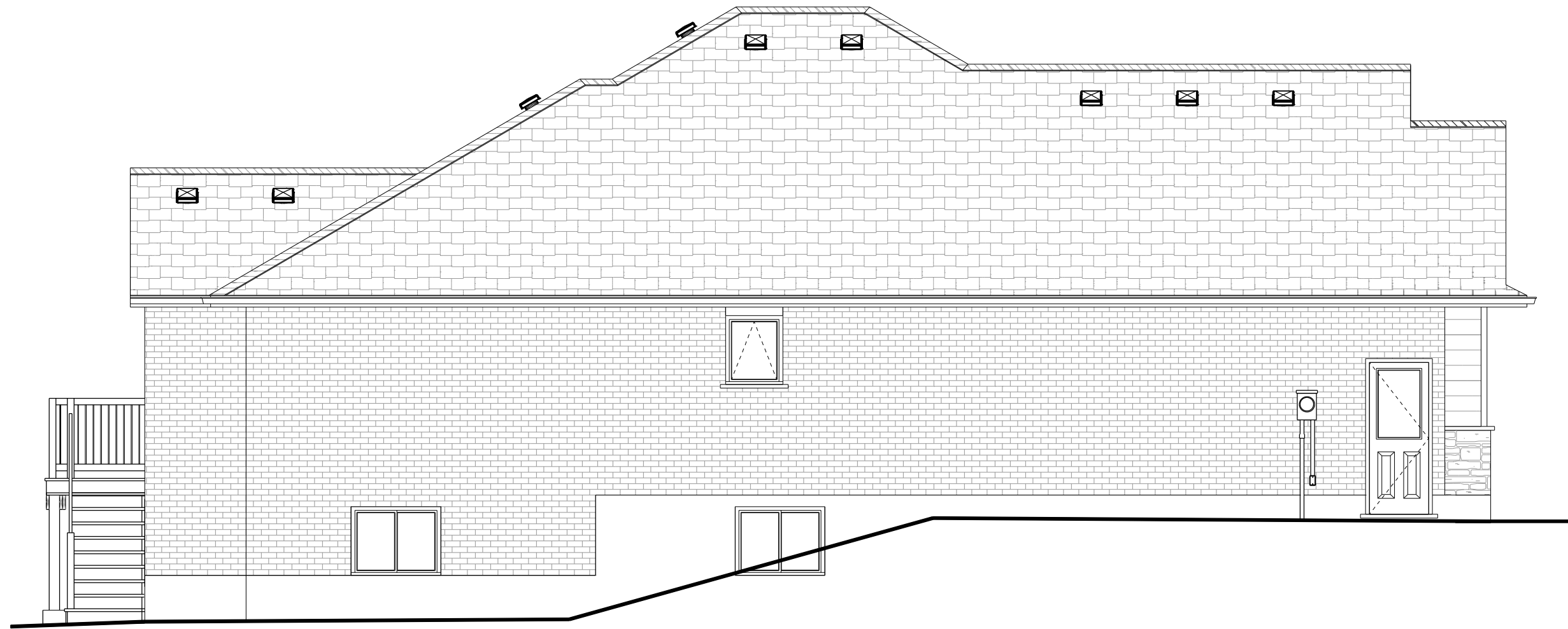
LEFT ELEVATION
