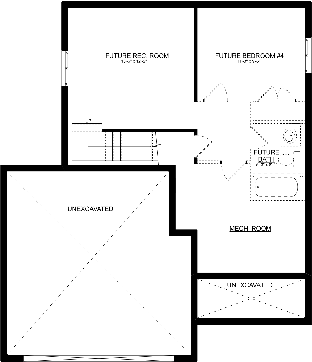
BASEMENT PLAN (NOT FINISHED)
