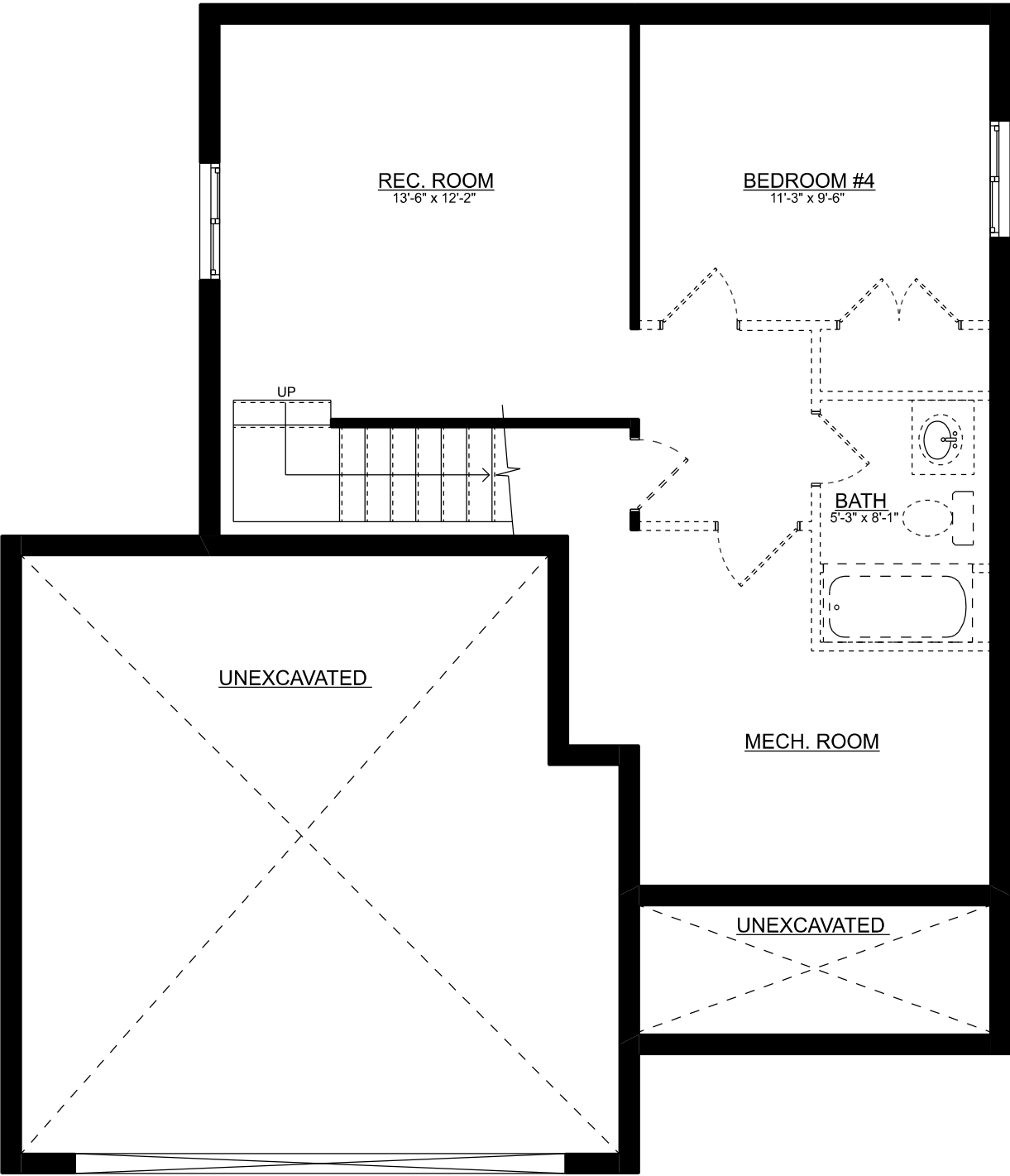
BASEMENT PLAN
