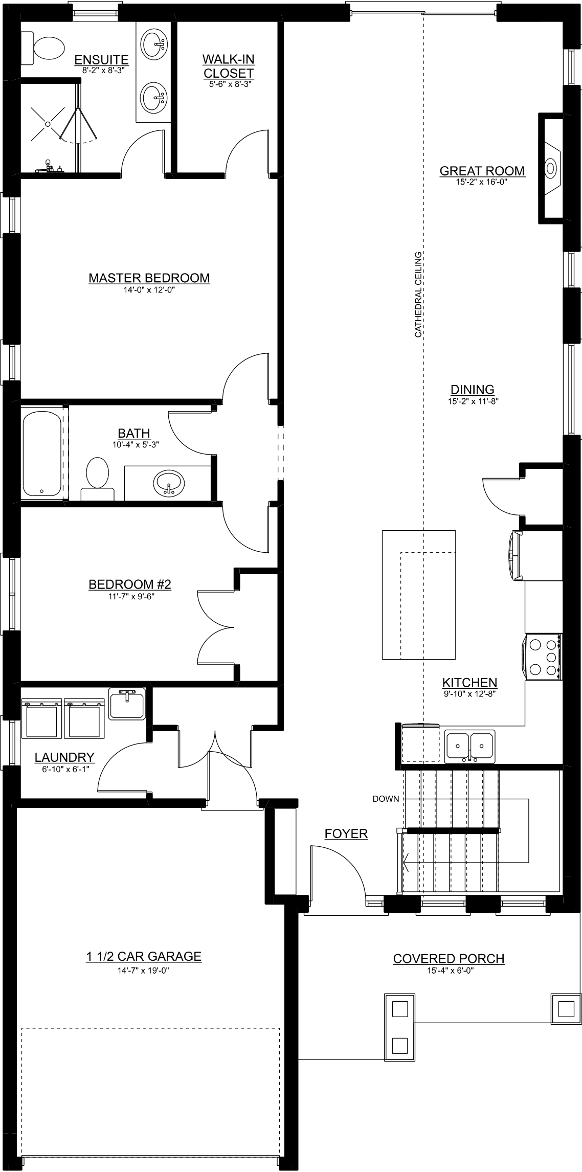
MAIN FLOOR PLAN
